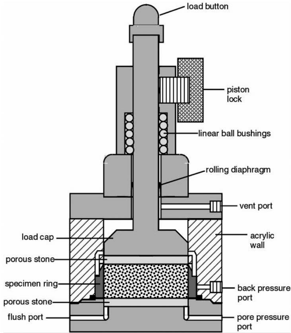
FIG. 2 Example of a CRS Consolidometer
